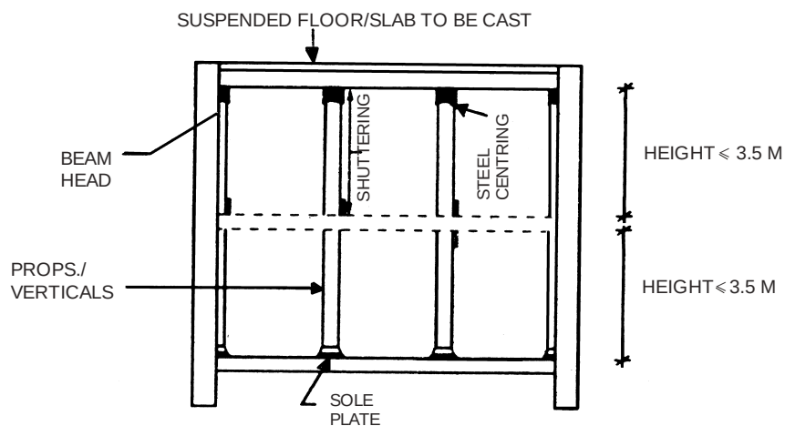
SUSPENDED FLOOR-MULTI STAGE SHUTTERING (VERTICAL SECTION)
