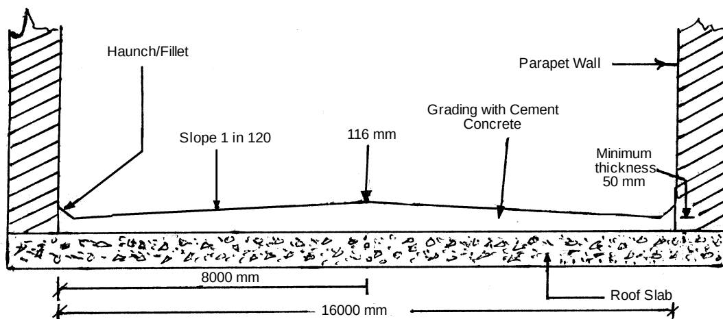
Fig. 22.8 : Grading Roof Slab with Cement Concrete
