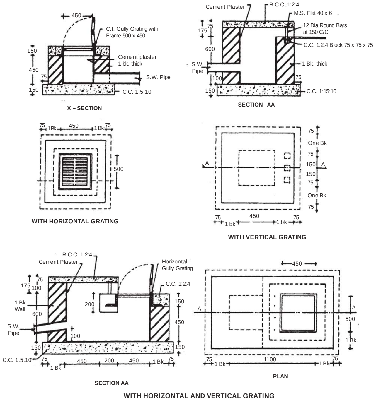
Fig. 19.14 : Road Gully Chamber
