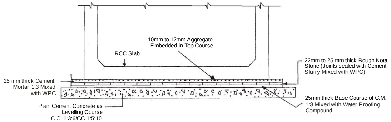
Fig. 22.1 : Waterproofing of Horizontal Surface of U.G. Structure
